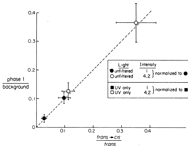
FIGURE 8 Phase I versus trans \rightarrow cis photoisomerization flux. Horizontal axis is 1 - \exp(-k_T) ; see text. Error bars reflect uncertainties in actinometric calibrations; see Methods. Vertical axis: phase I as fraction of agonist-induced conductance just before flash; see Figs. 6 and 7 and text. Error bars give SD (three to six cells per point). Trans -photoequilibrium solution of Bis-Q (usually 200 nM); voltage -150 mV; temperatures 10^\circ – 25^\circ C. Dashed line at 45^\circ gives prediction of trans \rightarrow cis photoisomerization hypothesis (see text).
